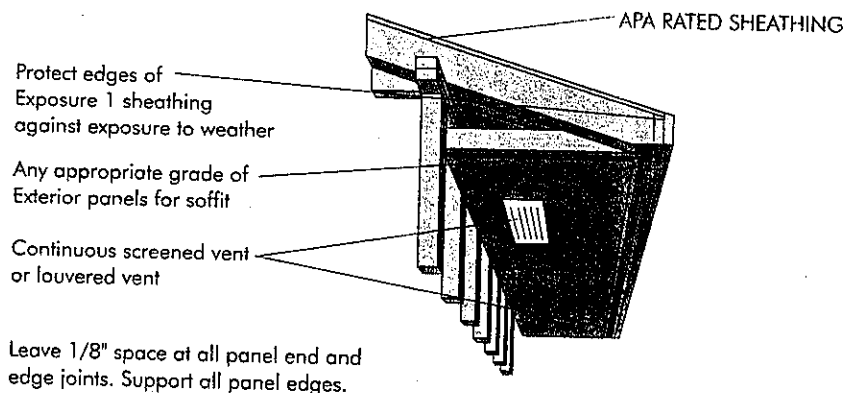
FIGURE 26 CLOSED SOFFIT
