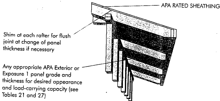
FIGURE 26 CLOSED SOFFIT
